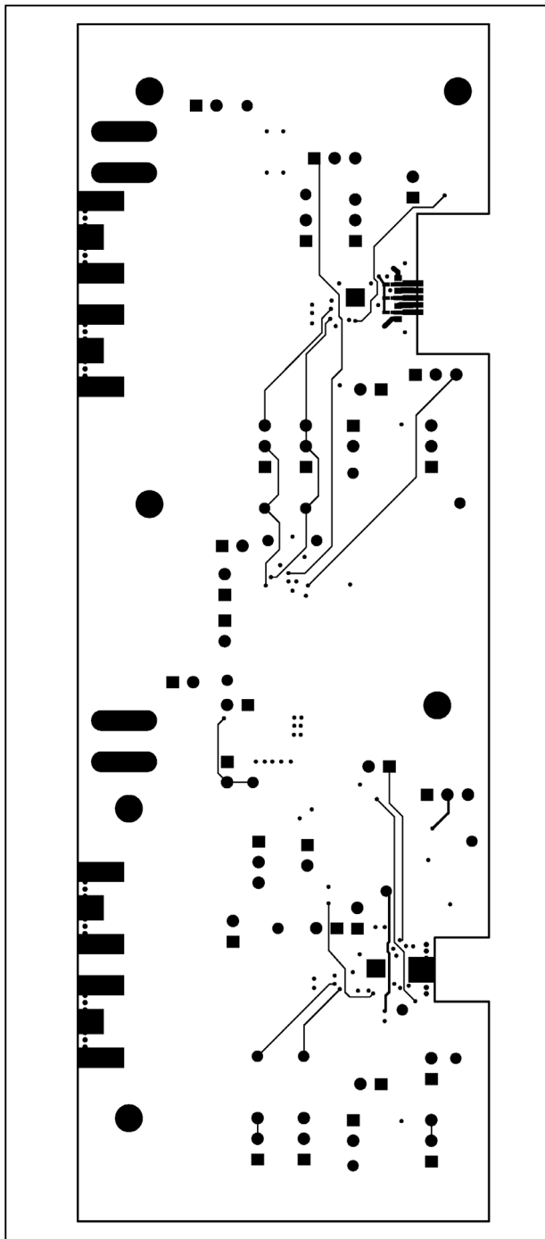
Figure 9. MAX3735A EV Kit PC Board Layout—Solder Side
