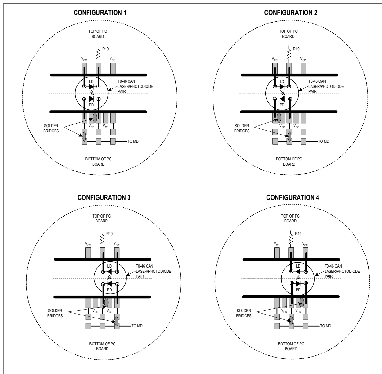
Figure 1. Attachment of Laser Diode/Monitor Diode to the MAX3735A EV Kit
